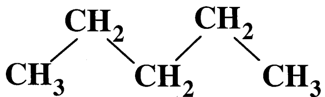
n-Pentane B.P. 36.1 °C
