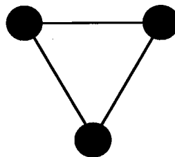
trigonal configuration
