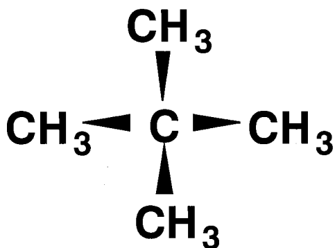
Neopentane B.P. 9.5 °C
